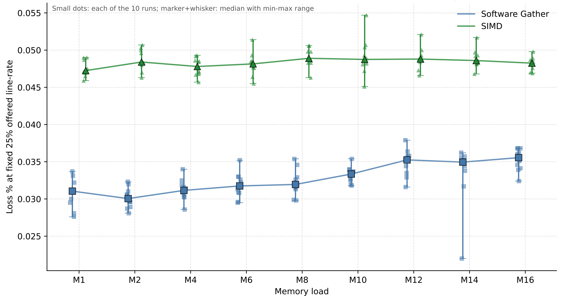
SIMD vs. Software Gather: loss at a fixed offered rate across memory loads
