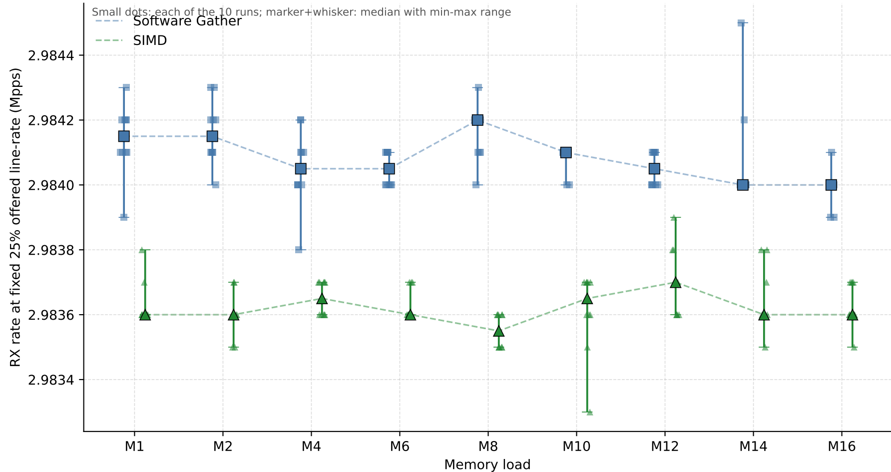
SIMD vs. Software Gather: RX rate at a fixed offered rate across memory loads
