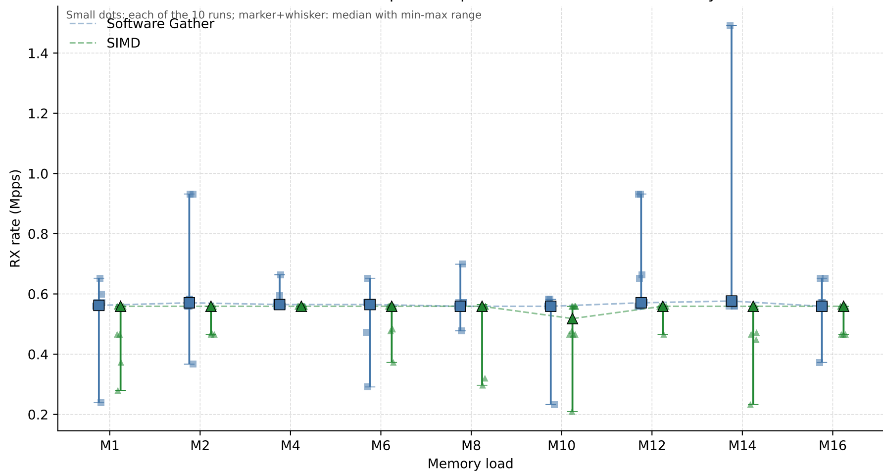
SIMD vs. Software Gather: per-run spread of RX rate across memory loads
