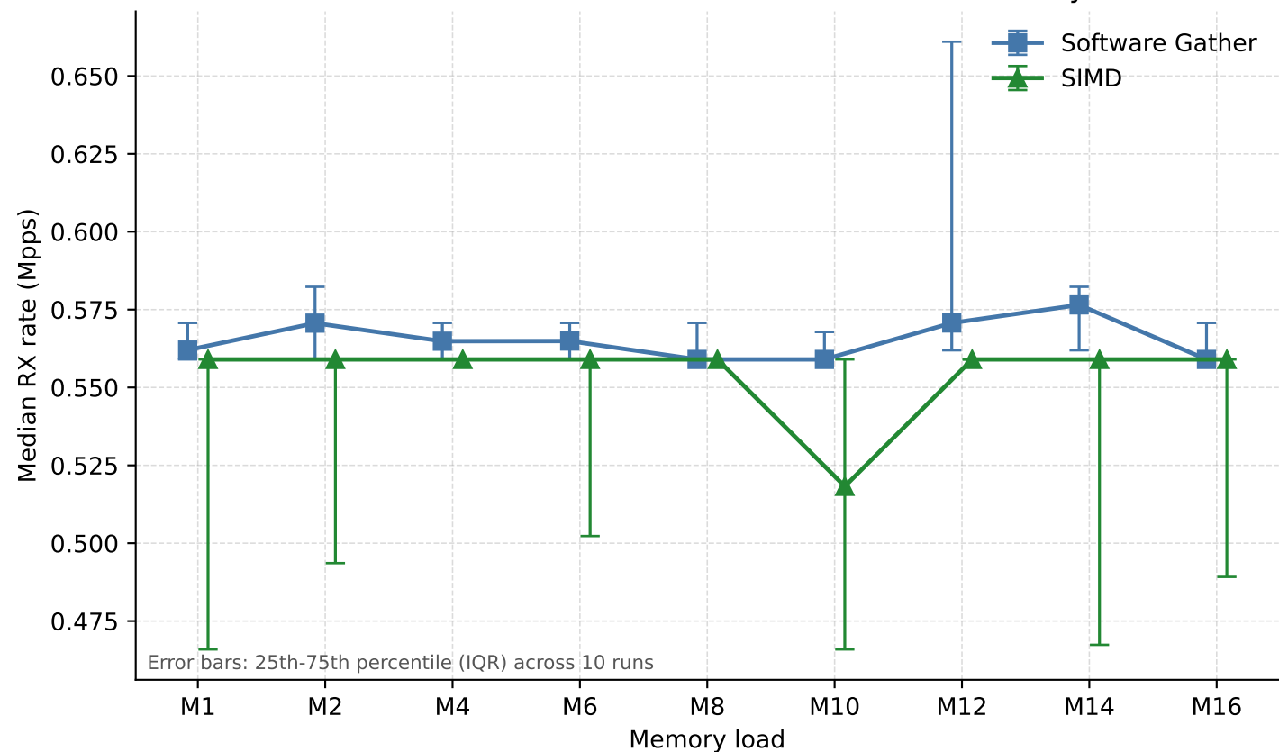
SIMD vs. Software Gather: median RX rate across memory loads
