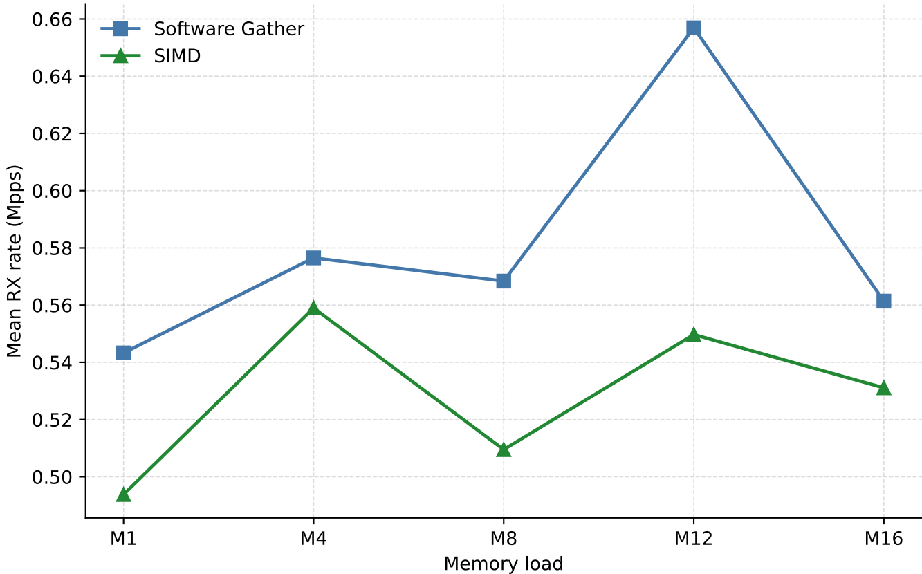
SIMD vs. Software Gather: mean RX rate across memory loads
