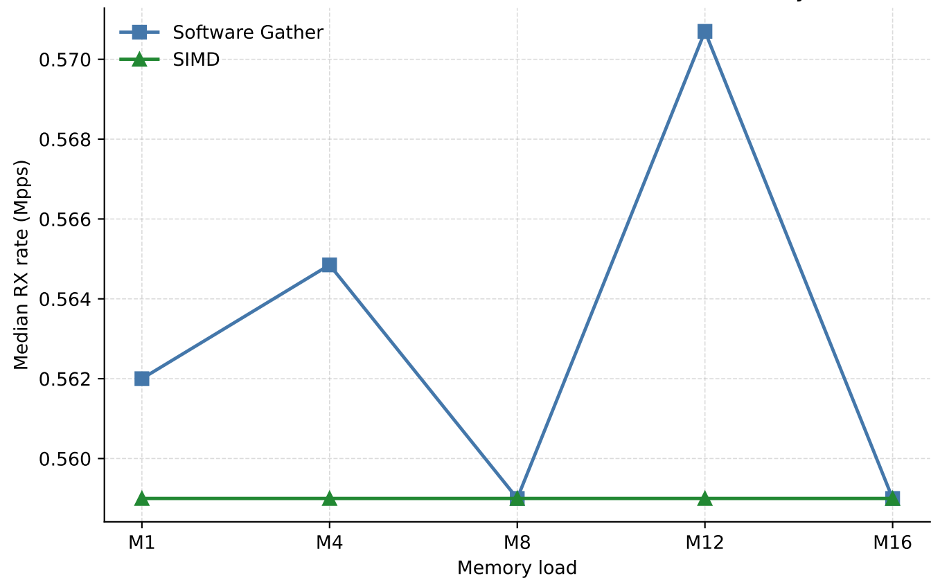
SIMD vs. Software Gather: median RX rate across memory loads
