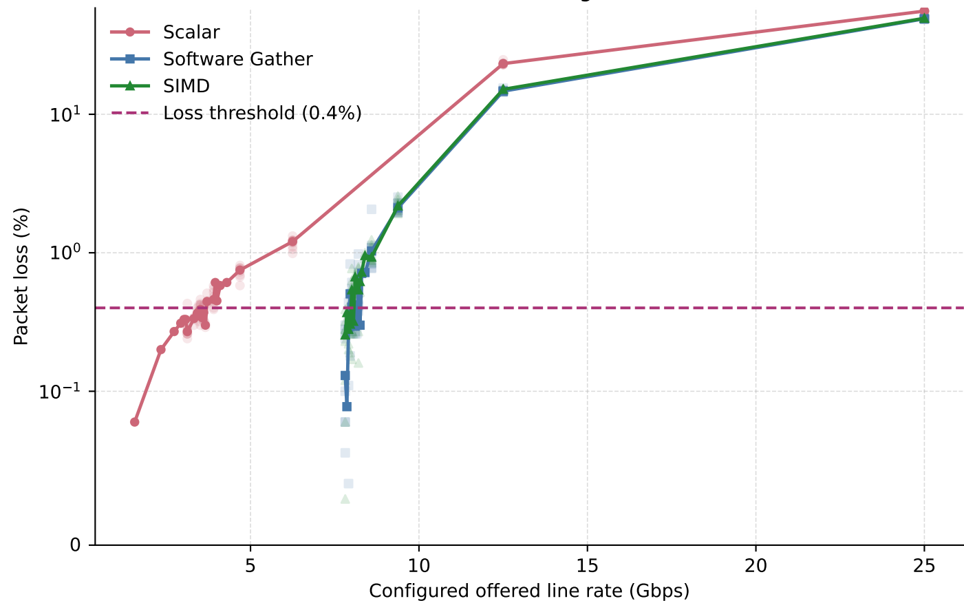
Packet loss versus configured line rate
