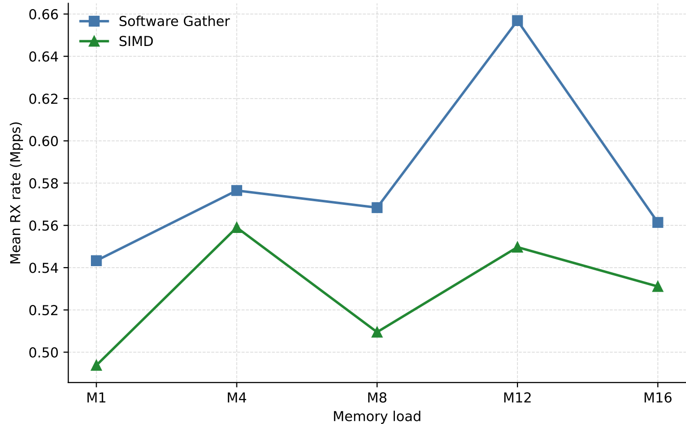
SIMD vs. Software Gather: mean RX rate across memory loads
