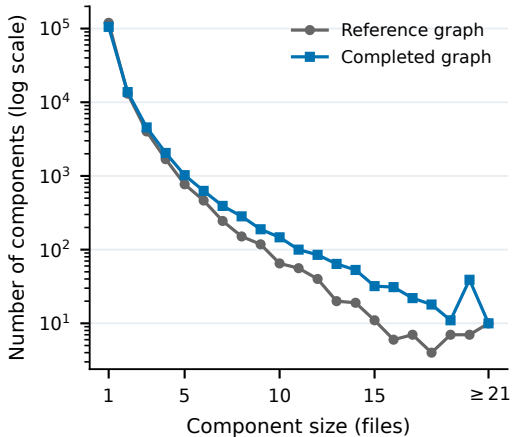
a Full-corpus component distribution
