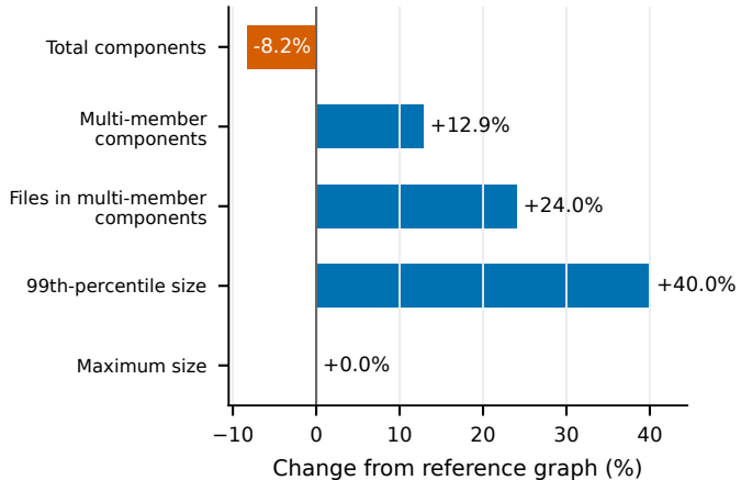
b Full-corpus graph completion
