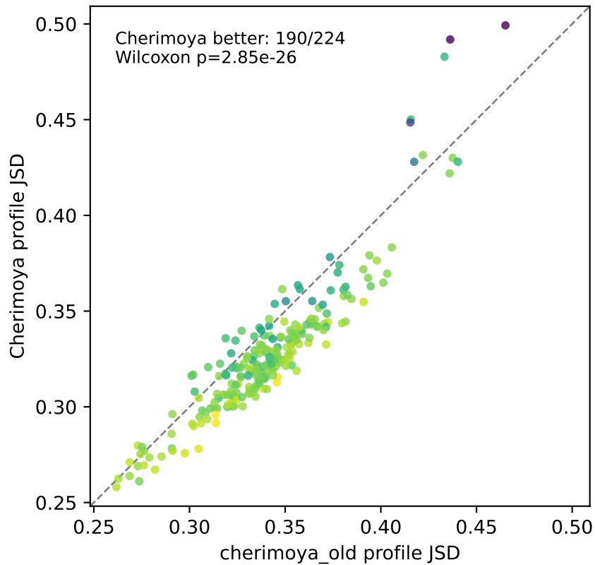
Profile JSD
