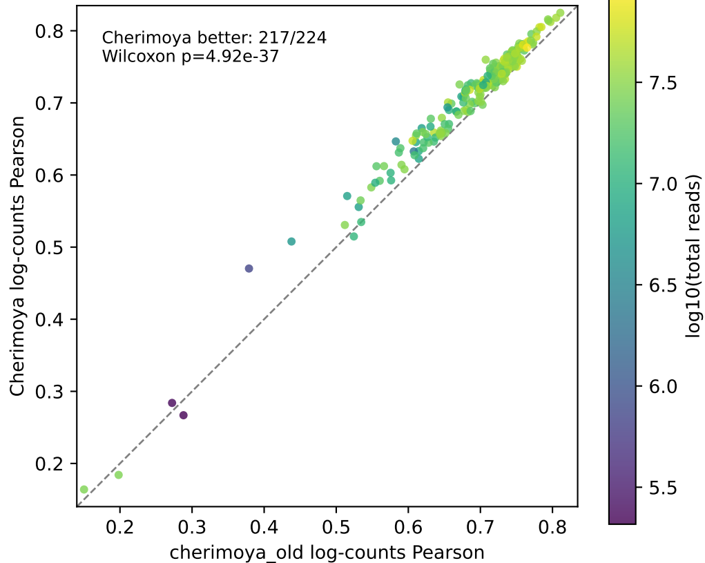
Log-counts Pearson
