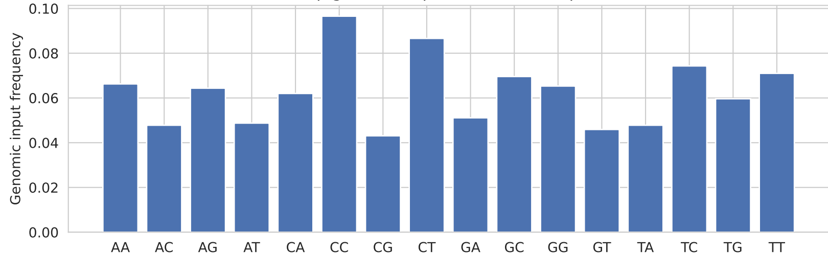
2114 bp genomic input dinucleotide spectrum
