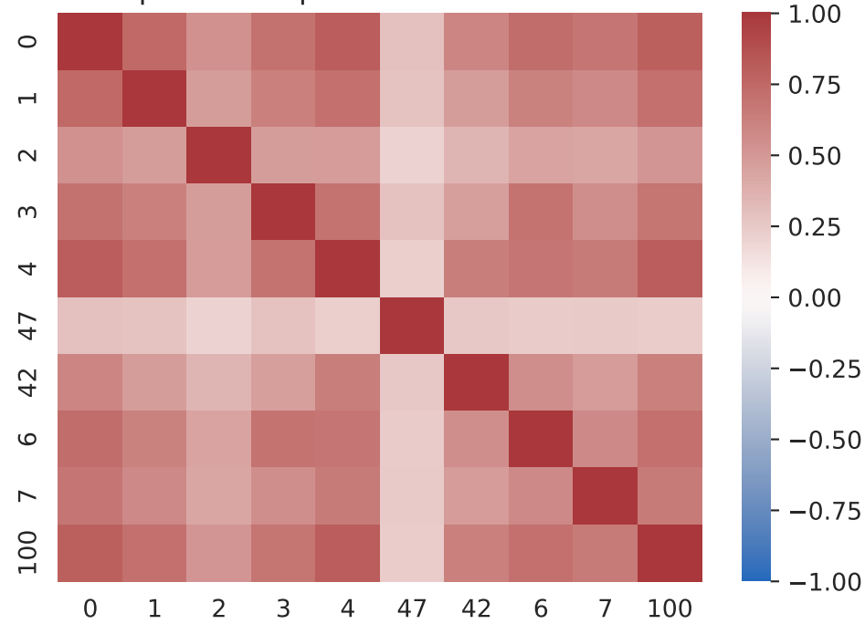
profile DeepLIFT seed correlation
