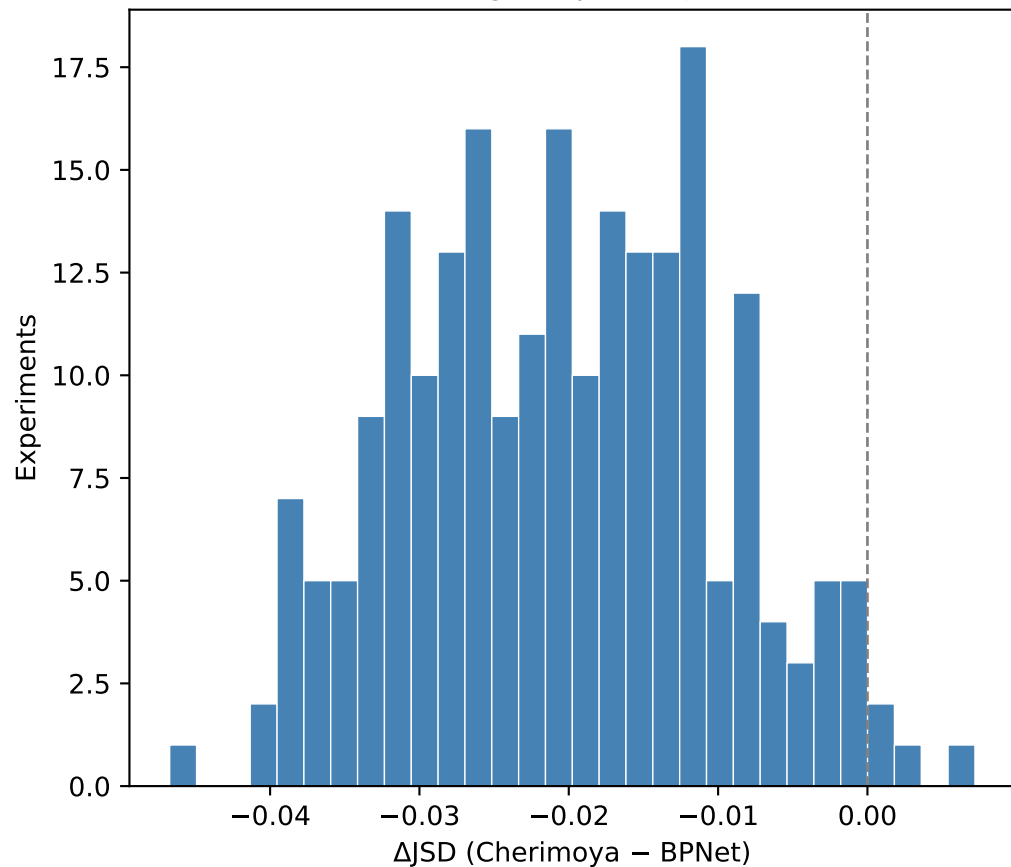
Change in profile JSD
