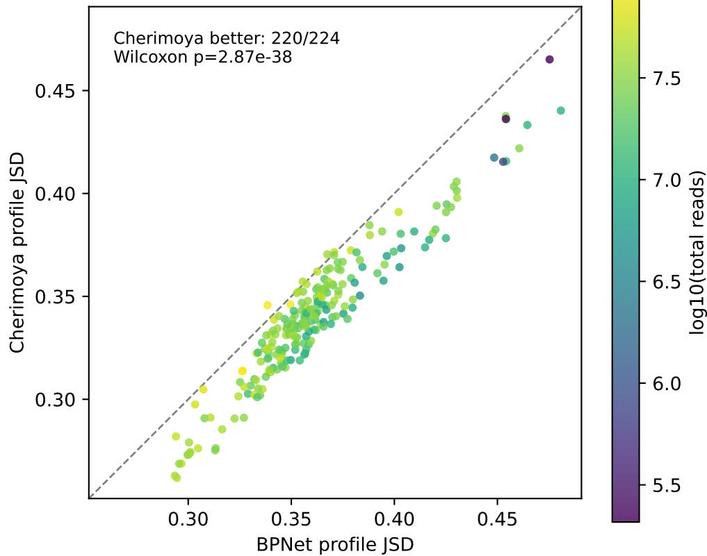
Profile JSD
