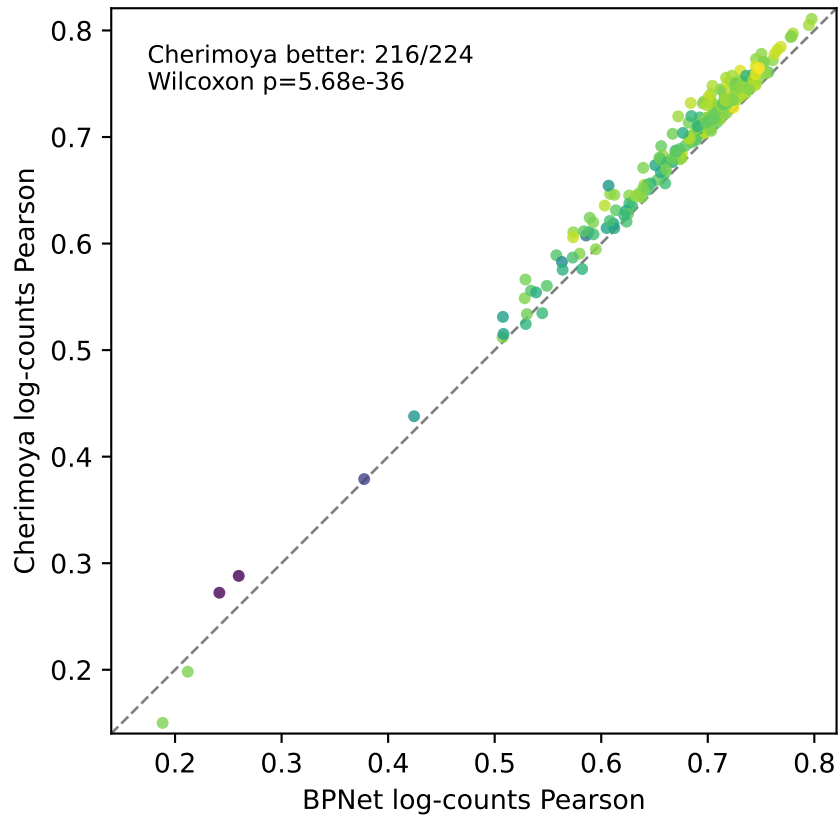
Log-counts Pearson
