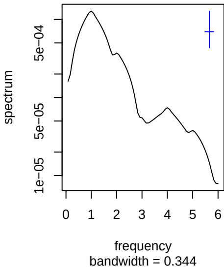
Series: res Smoothed Periodogram
