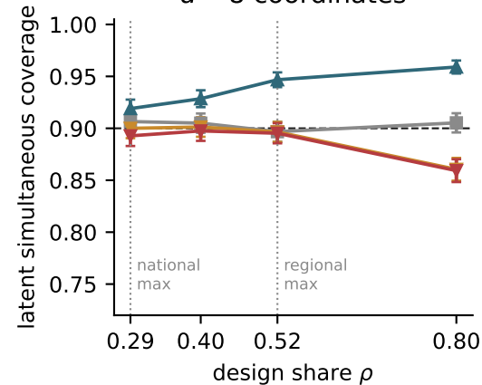
d = 8 coordinates
