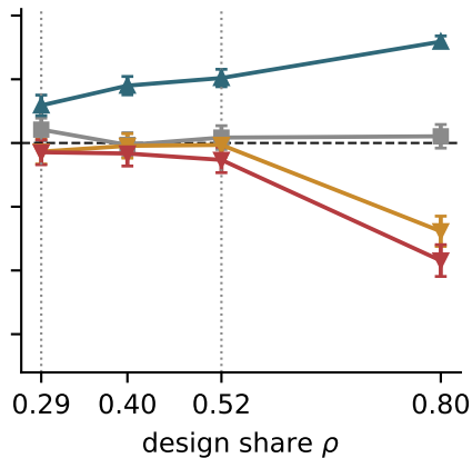
d = 24 coordinates
