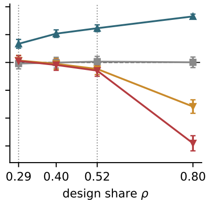
d = 48 coordinates
