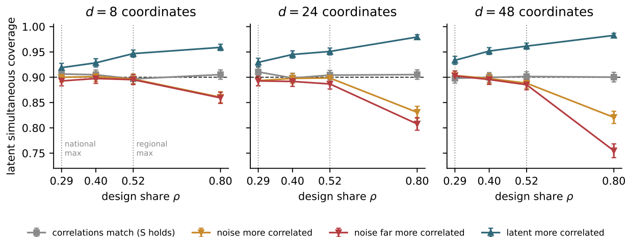
Figure 2: Latent simultaneous coverage of the oracle scale correction with exactly correct coordinate variances, by coordinate count, at K = 250 and nominal 90%. Bars are two Monte Carlo standard errors. Dotted verticals mark the largest design shares observed at the national and regional units.
