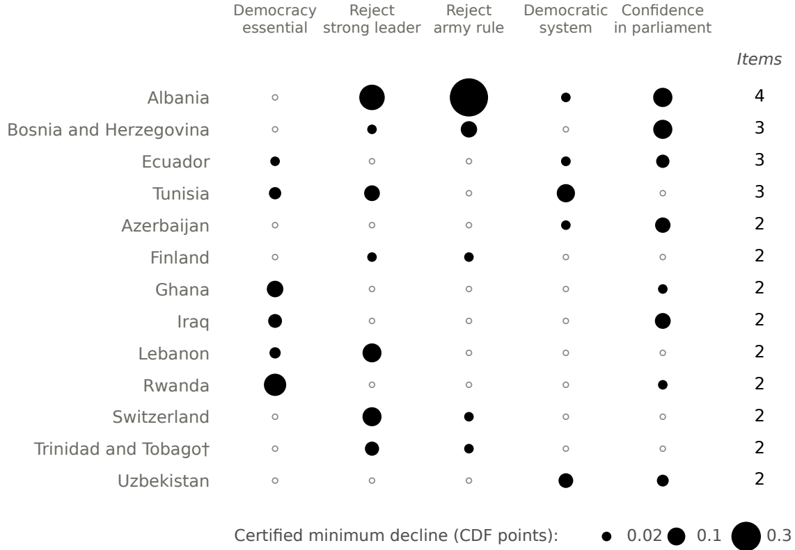
Figure 4: The thirteen-country descriptive co-certified core, by evidence strength (WVS 1981–2022; K = 59\text{--}77 per item). Twelve pass the valid \geq 2 -item partial-conjunction test; the dagger marks Trinidad and Tobago, which does not. Circle area is the persistent band’s simultaneous lower bound on the per-pair decline, in CDF points; open circles mark items that do not certify. The full thirty-eight-country matrix is in the Supplementary Material.
