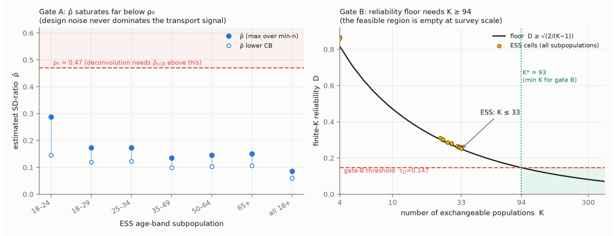
Figure 3: The two barriers, measured on real data. Left : across ESS age-band subpopulations \hat{\rho} saturates far below \rho_0 = 0.47 . Right : the finite- K reliability D sits on its distribution-free floor \sqrt{2/(K-1)} ; passing the reliability gate needs K \geq 94 , which cross-national surveys ( K \leq 33 ESS, \leq 105 WVS) reach only where—as on WVS—the design noise is too small for the need gate.
