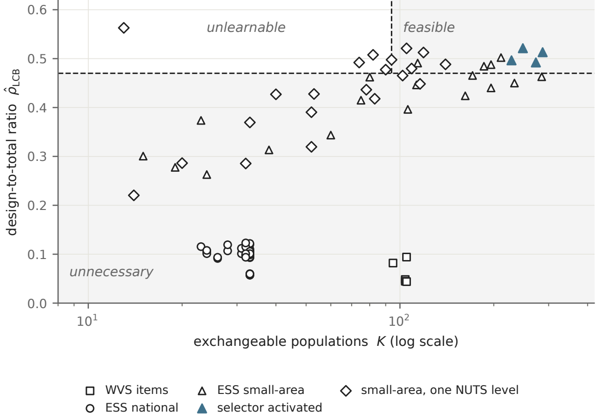
Figure 2: The feasibility frontier in the (K, \hat{\rho}_{LCB}) plane. Dashed boundaries: the need cutoff \rho_0 = 0.47 and the reliability floor K = 1 + 2/\tau_D^2 = 94 . Markers are real-data cells; the filled ones are the four where the frozen selector activated — only there are both boundaries crossed (e57; per-gate diagnostics in the Supplementary Material).
