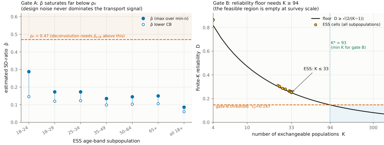
Figure 2: The two barriers at the national unit. Left : ESS age-band subpopulations (42 cells), \hat{\rho} vs \rho_0 . Right : D vs its floor \sqrt{2/(K-1)} ; only WVS full item-coverage sets reach K \geq 94 , and there the need gate fails.
