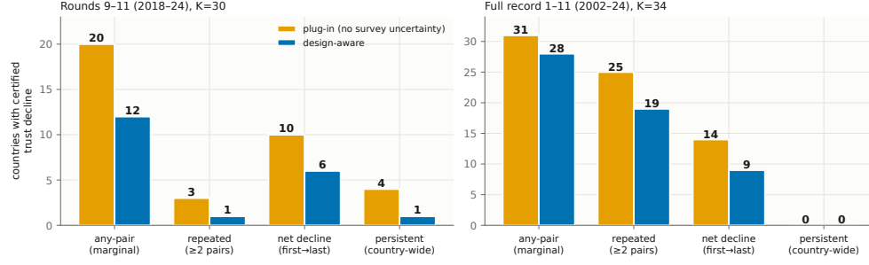
Figure 3: Certified declines collapse up the hierarchy ( \alpha = 0.10 ; plug-in and design-aware bars). Left , rounds 9–11 ( K = 30 ). Right , full record 2002–2024 ( K = 34 ).
