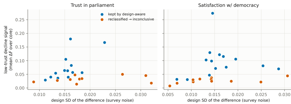
Figure S8: Relocated from the main text: countries certified by the marginal plug-in but inconclusive under the design-aware simultaneous band are the weak-signal, higher-noise cases; the apparent trend lies within the design uncertainty the survey warrants.
