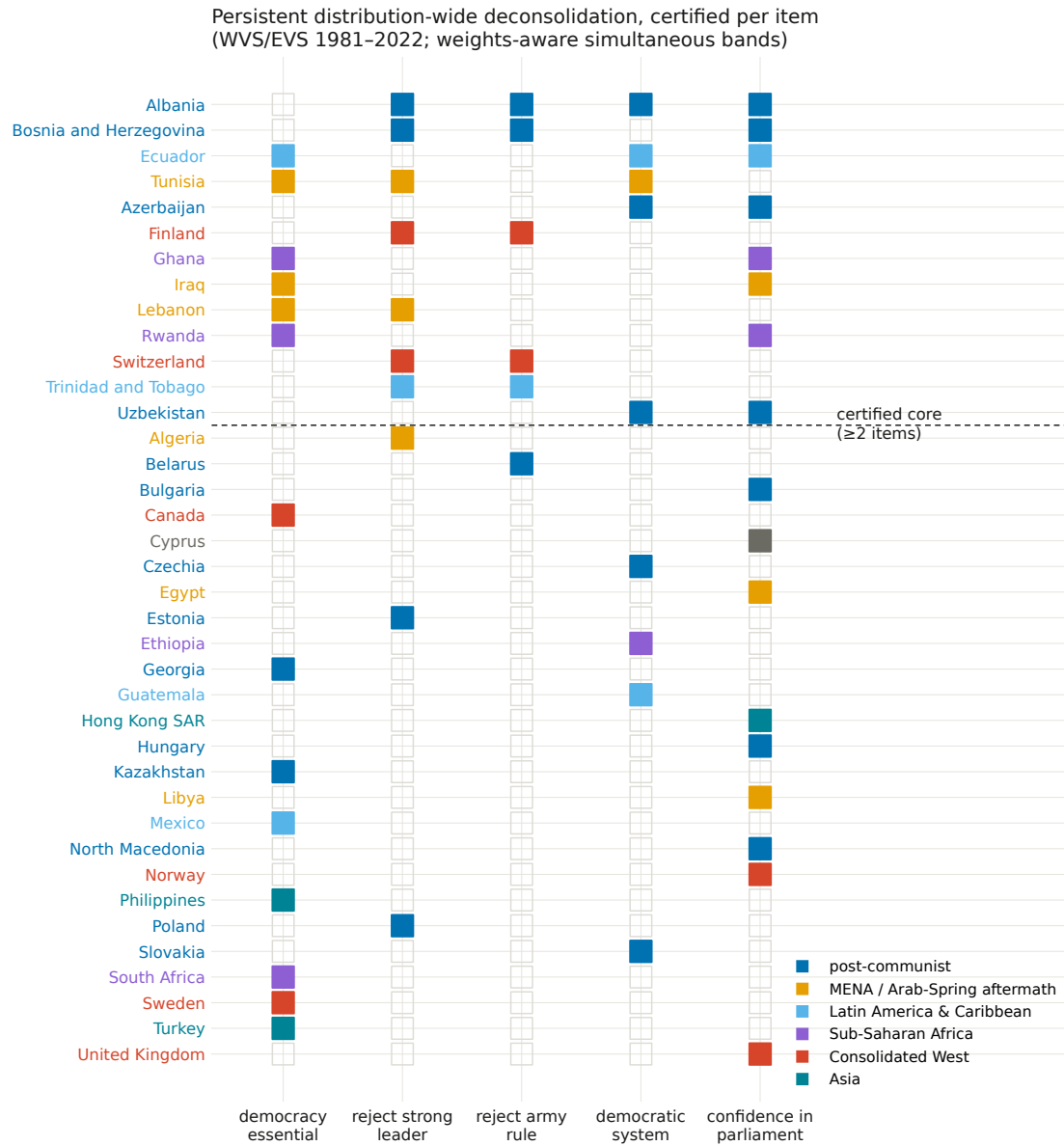
Figure 4: Co-certification across the five battery items (WVS/EVS 1981–2022; K = 59\text{--}77 per item). Countries above the dashed line form the \geq 2 -item certified core.
