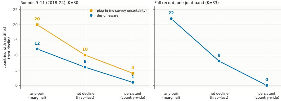
Figure 3: Certified declines collapse rung by rung ( \alpha = 0.10 ). Left, rounds 9–11 ( K = 30 ), with one path per inference layer; the headline sequence 20 \rightarrow 12 \rightarrow 6 \rightarrow 1 reads down the plug-in marker and then along the design-aware path. Right, the full record off one joint band ( K = 33 ), where the two layers coincide by construction and one path is drawn.
