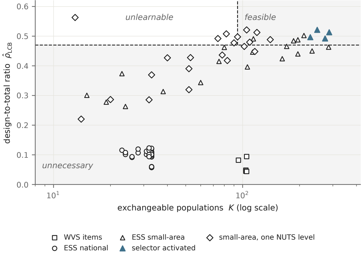
Figure 2: The feasibility frontier in the (K, \hat{\rho}_{\text{LCB}}) plane. Dashed boundaries: the need cutoff \rho_0 = 0.47 and the reliability floor K = 1 + 2/\tau_D^2 = 94 . Markers are real-data cells; the filled ones are the four where the frozen selector activated — only there are both boundaries crossed (per-gate diagnostics in the Supplementary Material).
