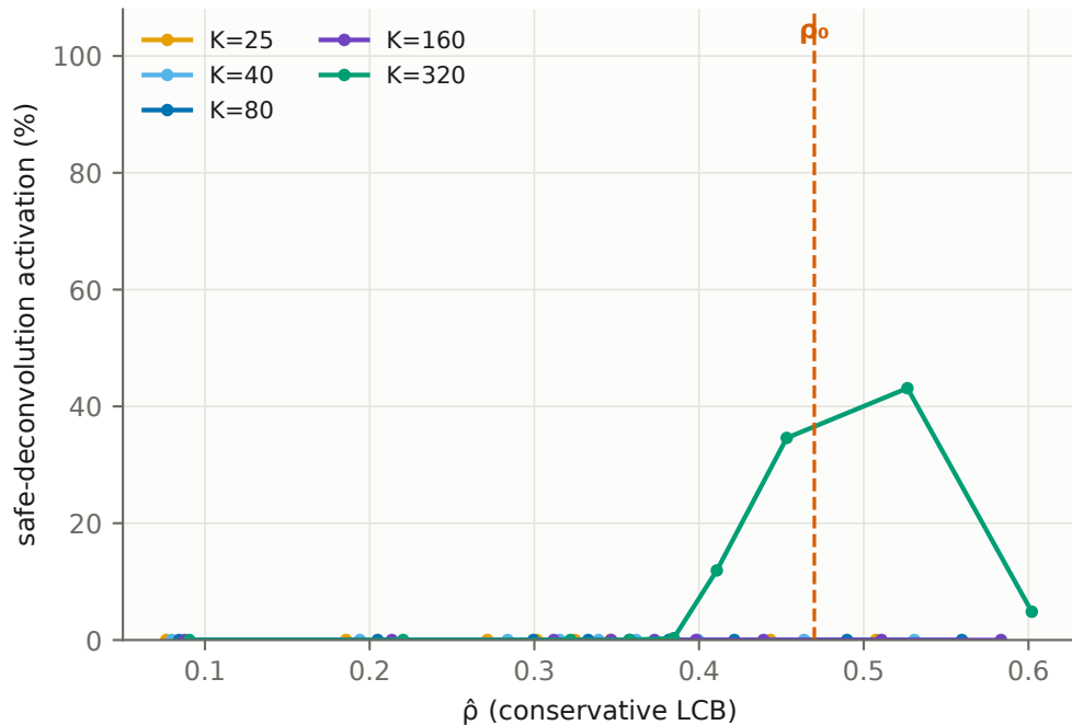
Efficient branch unlocks with K; small K: selector abstains
