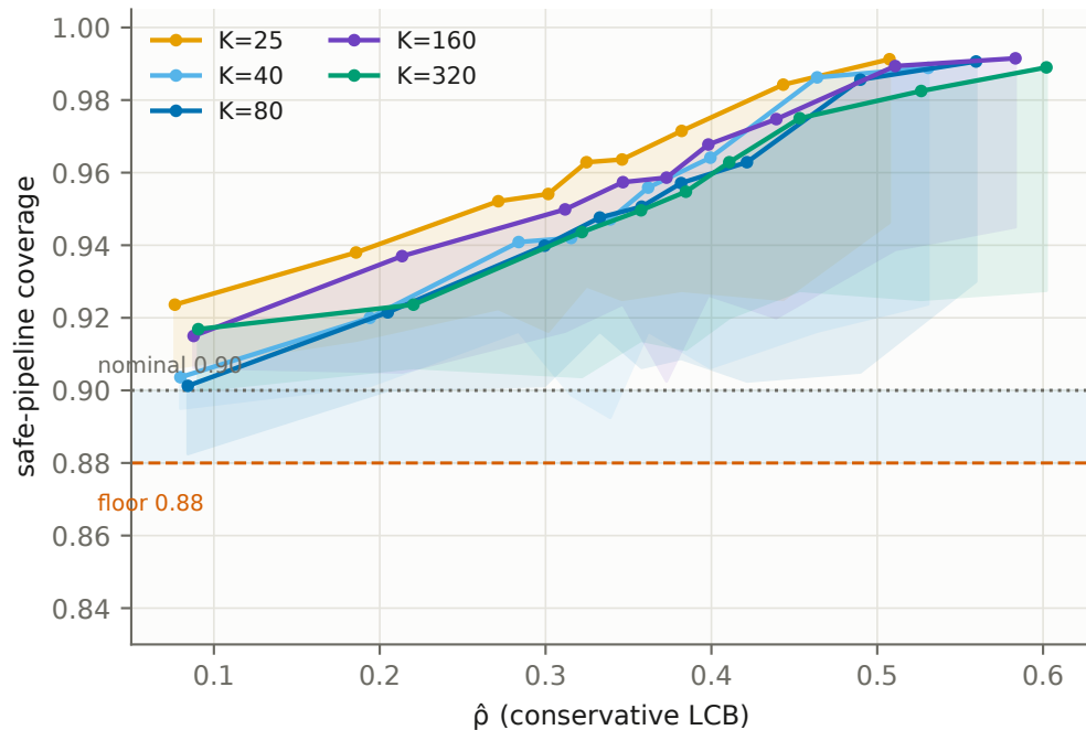
Coverage on the UNSEEN grid (10 new DGPs, new K, new \rho ) line = mean over families, shade = worst family
