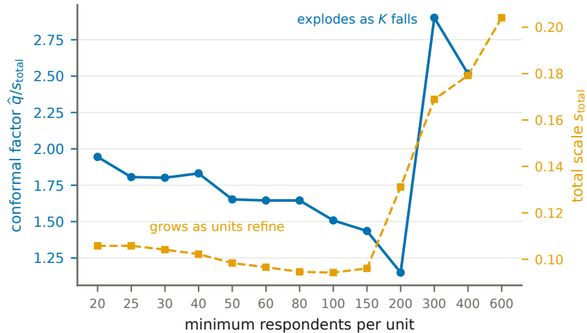
W = \hat{q} = \text{factor} \times s_{\text{total}}
