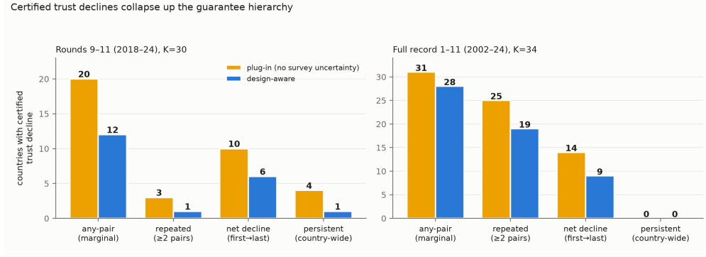
Figure 3: Certified trust declines collapse up the guarantee hierarchy ( \alpha = 0.10 ). Left , rounds 9–11 ( K = 30 ): 20 marginal \rightarrow 6 net \rightarrow one persistent (Greece). Right , full record 2002–2024 ( K = 34 ): 28 any-pair \rightarrow 9 net \rightarrow zero persistent.
