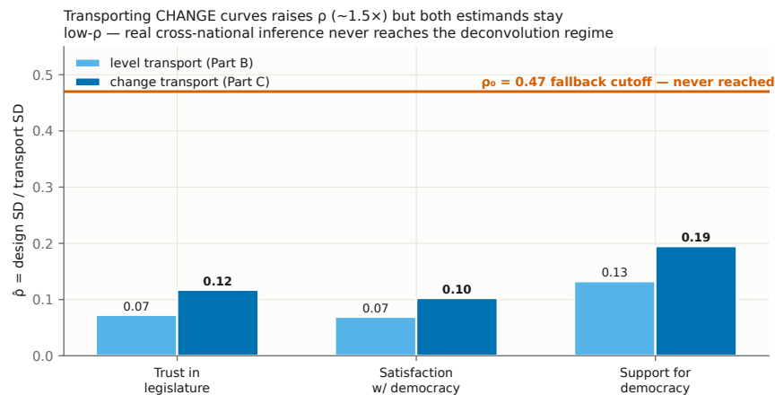
Figure S5: Design-to-total SD ratio \hat{\rho} , AmericasBarometer (levels and change; B = 200 design bootstrap). All country-outcomes sit well below \rho_0 = 0.47 ; the estimates are downward-biased floors.
