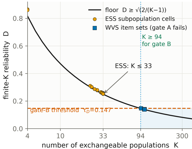
Gate B: reliability floor needs K \geq 94
