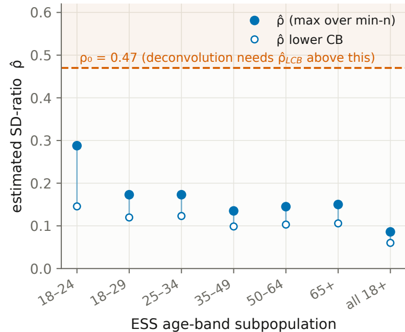
Gate A: \hat{\rho} saturates far below \rho_0
