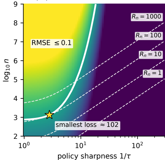
(a) population effect \theta (exact, HT)
