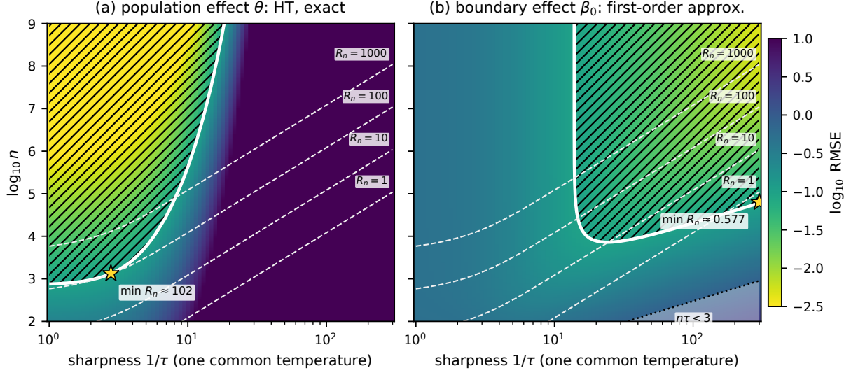
Figure 2: Root mean squared error (colour, \log_{10} scale) under one common temperature \tau for the design of Section 7: H \sim U(-1, 1) , \Delta(h) = h , g(h) = |h| , c(h) = 1 + |h| , unit noise. (a) Exact root mean squared error of the Horvitz–Thompson estimator of the population effect \theta . (b) First-order approximation, including the exact bias, to the root mean squared error of the estimator of Theorem 1 for the boundary effect \beta_0 ; the shaded region below the dotted line has n\tau < 3 , where Monte Carlo checks show the approximation overstates the error. Hatched regions, bounded by white curves, have root mean squared error at most 0.1. Dashed curves are levels of the cumulative exploration loss R_n = n\mathbb{E}[g(H)q_\tau(H)] . Stars mark the smallest loss that attains the precision on the plotted grid ( 1 \leq 1/\tau \leq 300 , 10^2 \leq n \leq 10^9 ). Panel (a) concerns one estimator under one outcome law; the lower bounds for all estimators are Theorems 2 and 3.
