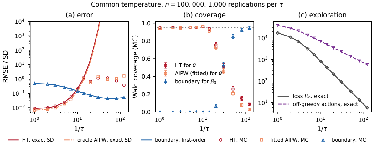
Figure 4: Common temperature at fixed n = 100,000 , 1,000 replications per temperature, same design as Figure 2. (a) Lines: exact standard deviation of the Horvitz–Thompson estimator and of an oracle augmented estimator that uses the true regression (a reference, not an estimator used in the simulation), both for \theta , and the first-order approximation to the root mean squared error of the boundary estimator of \beta_0 . Markers: Monte Carlo root mean squared error of the Horvitz–Thompson estimator, of the augmented estimator with a fitted linear working model, and of the boundary estimator. (b) Wald coverage with 95% Monte Carlo intervals. Boundary coverage is low while n\tau^3 is large, as Theorem 1(iv) requires. (c) Exploration loss R_n and expected number of off-greedy actions; lines are exact expectations, markers Monte Carlo.
