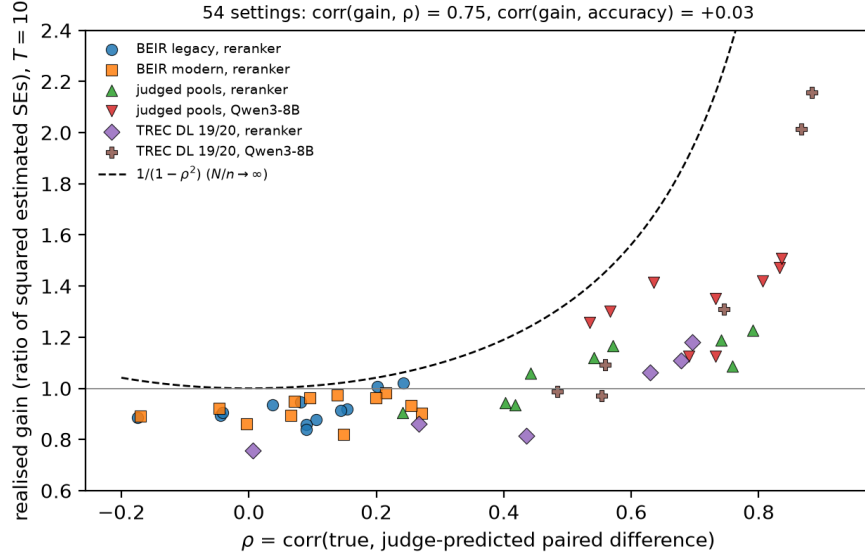
Figure 1: Realised PPI gain (ratio of squared estimated standard errors) at T = 10 against \rho , 54 settings, cross-fitted \lambda . The dashed curve is 1/(1 - \rho^2) . Gains track \rho (0.75) and not accuracy (0.03).
