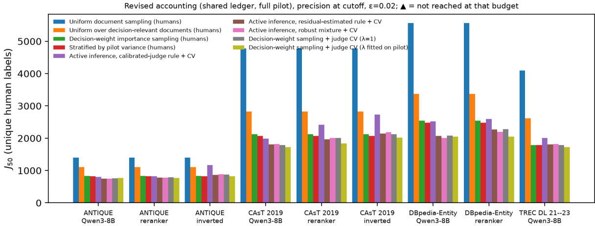
Figure 4: J_{50} by method (precision at cutoff, \varepsilon = 0.02 ). The bulk of the saving comes from decision-weight importance sampling; the judge adds a judge- and collection-dependent increment as a control variate; the calibrated-judge active rule is the only arm badly hurt by an adversarial judge.
