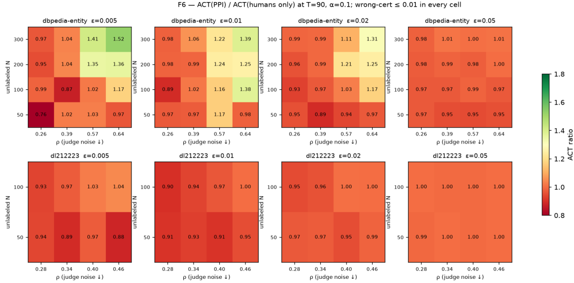
Figure 2: Mechanism map: ACT(PPI)/ACT(humans) at T = 90 over \rho (judge-label noise), unlabeled pool size and \epsilon ; wrong-certificate rate \leq 0.01 in every cell. Gains appear only for \rho \geq 0.57 and \epsilon \leq 0.02 , grow with N_{\text{unlab}} , and are absent at N_{\text{unlab}} = 50 and at \epsilon = 0.05 .
