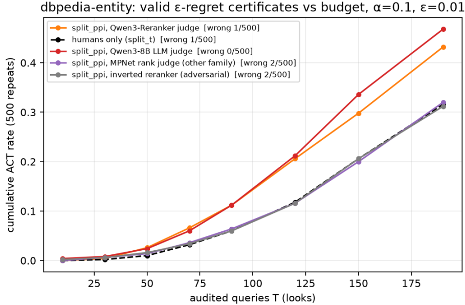
Figure 3: Cumulative ACT rate of the split certificate against the audit budget on DBpedia-Entity (500 repeats, \epsilon = 0.01 ). Judges change the slope, not the validity: wrong certificates \leq 2/500 for every curve, including the inverted (adversarial) judge.
