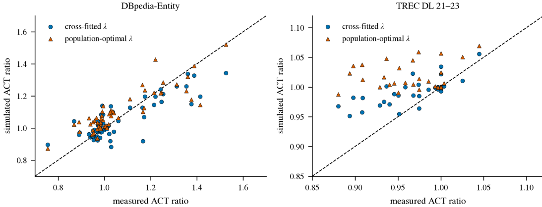
Figure 7: Simulated against measured ACT ratio, T = 90 , every cell of Figure 2; circles use the cross-fitted \lambda of the implementation, triangles the population-optimal \lambda . Left DBpedia-Entity, right TREC DL 2021–23.
