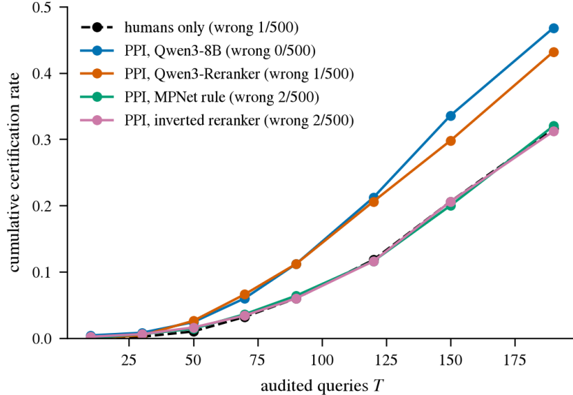
Figure 6: Cumulative ACT rate of the split certificate against the audit budget on DBpedia-Entity (500 repeats, \varepsilon = 0.01 ). Judges change the slope, not the validity: wrong certificates \leq 2/500 for every curve, including the inverted (adversarial) judge.
