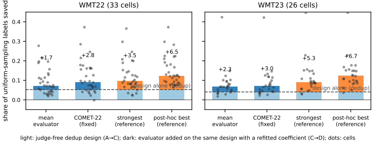
Figure 1: Same-condition decomposition of the saving over uniform sampling (medians over informative cells; same menus, pilot, \varepsilon and simulated audits). Light: the judge-free dedup design, s_D = 1 - C/A ; dark: an evaluator added on the same design with a refitted coefficient, (1 - s_D)h with h = 1 - D/C , so the bar’s height is s_{\text{total}} = 1 - D/A . Mean evaluator and the pre-fixed COMET-22 are strategies an auditor can run; the strongest evaluator of the year (MetricX-XXL, XCOMET-XXL) and the post-hoc best are chosen from the outcome and shown as reference. Dots: cells. WMT22: 33 cells, 300 audits, 31 metrics; WMT23: 26 cells, 300 audits, 42 metrics.
