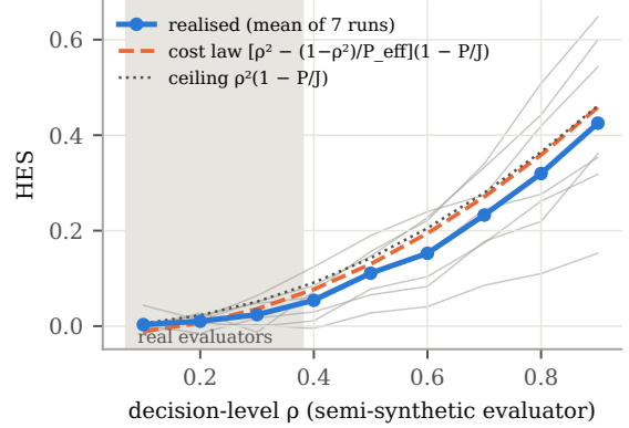
Figure 5: Realised HES of semi-synthetic evaluators with a set decision-level \rho (grey: individual runs) against the cost law (2) and its oracle- \lambda ceiling. Shaded: the range of the real evaluators. Identical output strings of an item share one noise draw (an earlier version drew noise per output, which left the never-sampled known-zero items with a non-zero prediction term of at most 6 \times 10^{-4} ; the correlation was 0.975 and the savings 11% / 32%).
