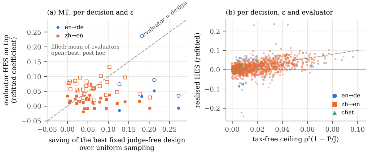
Figure 2: The 30 two-system WMT22 decisions at 300 audits per cell (the text of §3.2 reports the 2,000-audit re-run, 36 cells, whose medians agree). (a) The 33 MT decision- \epsilon cells (19 decisions) in which at least 30% of the uniform-sampling cost falls after the pilot: saving of the best fixed judge-free design over uniform sampling against the HES of the evaluators on top of it (refitted coefficient; filled: mean of the 34 evaluators, open: best, post hoc). (b) Every informative decision, \epsilon and evaluator, MT and chat (1,158 points): realised HES against the tax-free approximation \rho^2(1 - P/J) of (2), with the pilot-median \rho .
