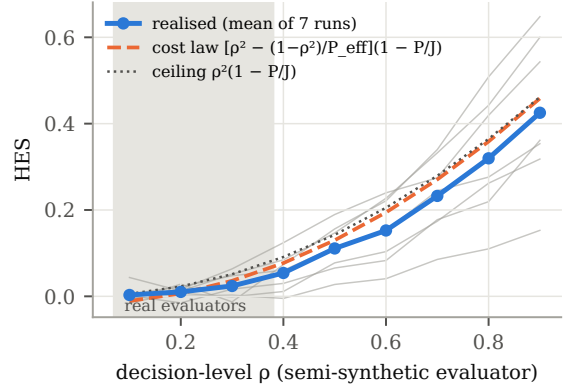
Figure 5: Realised HES of semi-synthetic evaluators with a set decision-level \rho (grey: individual runs) against the cost law (2) and its oracle- \lambda value. Shaded: the range of the real evaluators. Identical output strings of an item share one noise draw (an earlier version drew noise per output, which left the never-sampled known-zero items with a non-zero prediction term of at most 6 \times 10^{-4} ; the correlation was 0.975 and the savings 11% / 32%).
