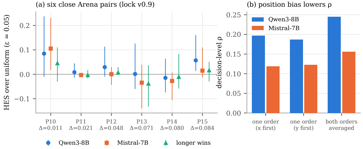
Figure 6: (a) HES over uniform sampling of three evaluators on six close LMArena pairs ( \Delta : human win-rate gap; pilot 50, \varepsilon = 0.05 ; 95% intervals). (b) Decision-level \rho with one presentation order and with both orders averaged.
