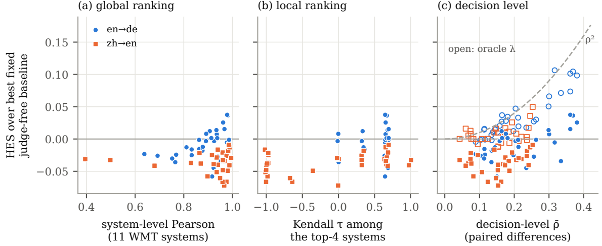
Figure 4: Thirty WMT22 metric variants at three levels of quality against their realised human-evidence saving over the best fixed judge-free baseline (pilot 50, mean over \varepsilon \in \{0.01, 0.02\} ). (c) open markers: the same metrics with the population-optimal (oracle) correction coefficient; dashed: \rho^2 , the asymptotic saving. REUSE (negative system-level correlation; switched off by \lambda \geq 0 ) is omitted.
