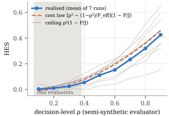
Figure 5: Realised HES of semi-synthetic evaluators with a set decision-level \rho (grey: individual runs) against the cost law (2) and its oracle- \lambda value. Shaded: the range of the real evaluators. Identical output strings of an item share one noise draw (an earlier version drew noise per output, which left the never-sampled known-zero items with a non-zero prediction term of at most 6 \times 10^{-4} ; the correlation was 0.975 and the savings 11% / 32%).
