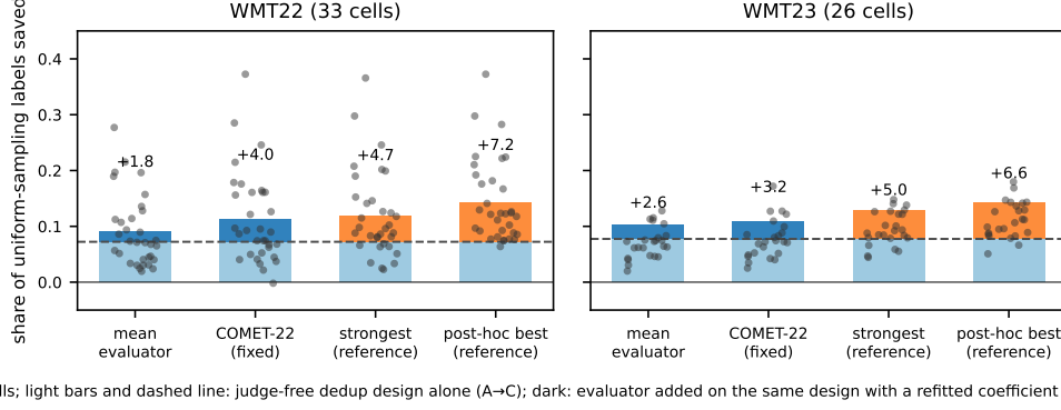
Figure 1: Same-condition decomposition of the saving over uniform sampling (same menus, pilot, \varepsilon and simulated audits). Per cell, s_{\text{total}} = 1 - D/A = s_D + (1 - s_D)h with s_D = 1 - C/A the judge-free dedup design’s share (light) and (1 - s_D)h , h = 1 - D/C , the evaluator’s on the same design with a refitted coefficient (dark); the bars stack the means over informative cells of the two parts, so their sum is the mean total (medians, which the text reports, do not add). Mean evaluator and the pre-fixed COMET-22 are strategies an auditor can run; the strongest evaluator of the year (MetricX-XXL, XCOMET-XXL) and the post-hoc best are chosen from the outcome and shown as reference. Dots: cells. WMT22: 33 cells, 300 audits, 31 metrics; WMT23: 26 cells, 2,000 audits, 42 metrics.
