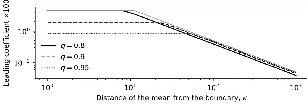
Figure S2: Leading coefficient L_q(\kappa) of the worst-case radius correction, times 100, when the mean lies at distance at least \kappa x^{1/2} from the boundary (Theorem 5), for q = 0.8 (solid), 0.9 (dashes) and 0.95 (dots), with the upper bound \min\{c_q, (\kappa^2 + 1)^{1/2} - \kappa\} from Theorems 3 and 4 (grey). Both axes are logarithmic.
