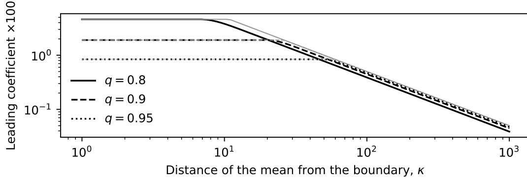
Fig. 1. Leading coefficient L_q(\kappa) of the worst-case radius correction, times 100, when the mean lies at distance at least \kappa x^{1/2} from the boundary (Theorem 3), for q = 0.8 (solid), 0.9 (dashes) and 0.95 (dots), with the upper bound \min\{c_q, (\kappa^2 + 1)^{1/2} - \kappa\} from Theorems 1 and 2 (grey). Both axes are logarithmic.
