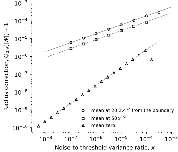
Figure S2: Radius correction Q_{0.9}(|W|) - 1 against x on logarithmic axes, for laws with noisy coverage exactly 0.9: mean at 20.2 x^{1/2} from the boundary (circles), at 50 x^{1/2} (squares) and mean zero (triangles), with c_{0.9} x^{1/2} (solid), L_{0.9}(50) x^{1/2} (dashes) and 0.024 x (dots). Only positive corrections are shown.
