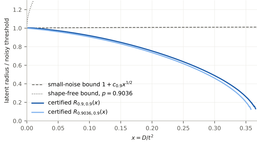
Figure S3: Certified sharp radius R_{p,0.9}(x) for p = 0.9 and for the order-statistic level p = 0.9036 , with the small-noise bound of Theorem 1 and the shape-free bound 1 + x^{1/2}z_{1-(p-q)/2} , which follows from |W| \leq |V| + |e| .
