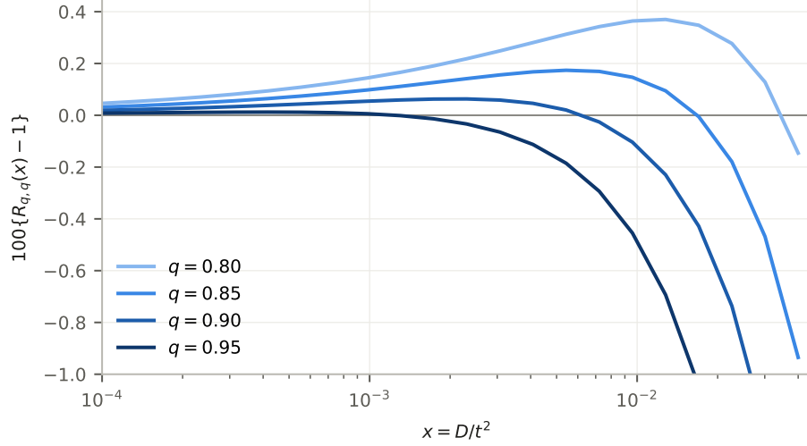
Figure 1: Sharp latent radius relative to the noisy threshold, 100\{R_{q,q}(x) - 1\} , for four coverage levels. Above zero the noisy threshold must be widened; below zero it may be shrunk.
