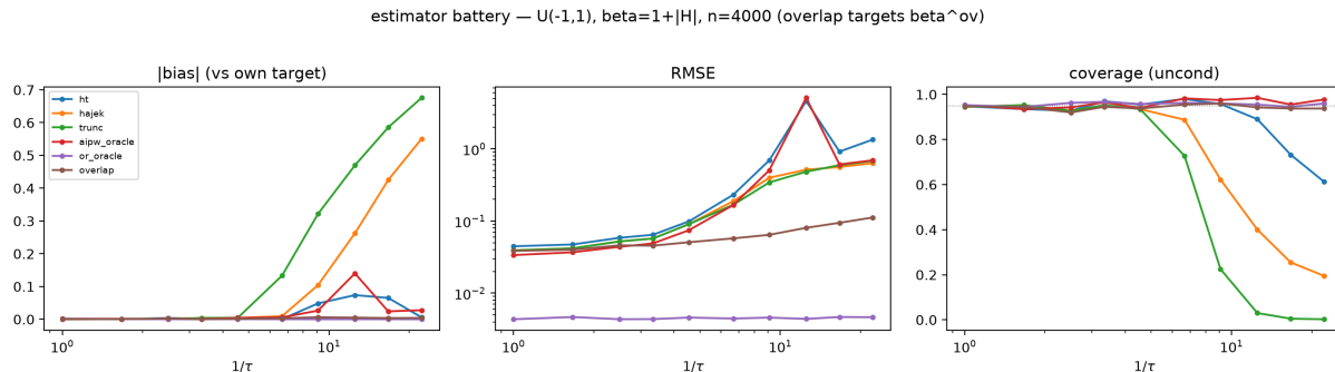
Figure 4: Estimator battery on the continuous-boundary design, n = 4,000 (bias against each estimator’s own target; the overlap estimator targets \beta^{\text{ov}} ). The numerical values quoted in the text are for n = 32,000 , the largest cell of the grid.
