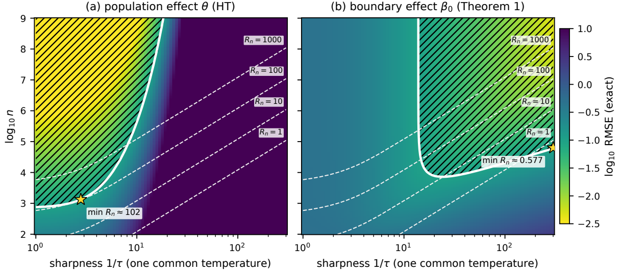
Figure 2: Exact root mean squared error (colour, \log_{10} scale) under one common temperature \tau for the design of Section 7: H \sim U(-1, 1) , \Delta(h) = h , g(h) = |h| , c(h) = 1 + |h| , unit noise. (a) The Horvitz–Thompson estimator of the population effect \theta . (b) The estimator of Theorem 1 for the boundary effect \beta_0 , including its bias. Hatched regions, bounded by white curves, have root mean squared error at most 0.1. Dashed curves are levels of the cumulative exploration loss R_n = n\mathbb{E}[g(H)q_\tau(H)] . Stars mark the smallest loss that attains the precision on the plotted grid ( 1 \leq 1/\tau \leq 300 , 10^2 \leq n \leq 10^9 ). Panel (a) concerns one estimator under one outcome law; the lower bounds for all estimators are Theorems 2 and 3.
