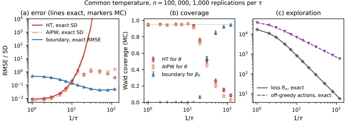
Figure 4: Common temperature at fixed n = 100,000 , 1,000 replications per temperature, same design as Figure 2. (a) Lines: exact standard deviation of the Horvitz–Thompson and augmented (true regression) estimators of \theta , and exact root mean squared error of the boundary estimator of \beta_0 . Markers: Monte Carlo root mean squared error; the augmented estimator uses a linear working model. (b) Wald coverage with 95% Monte Carlo intervals. Boundary coverage is low while n\tau^3 is large, as Theorem 1(iv) requires. (c) Exploration loss R_n and expected number of off-greedy actions; lines are exact, markers Monte Carlo.
