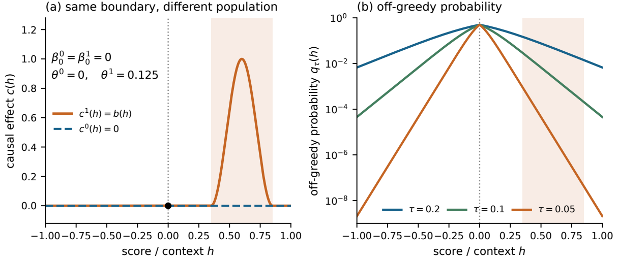
Figure 1: The separation construction, with H \sim U(-1, 1) , g(h) = |h| , u_1 = 0.35 , u_2 = 0.85 , and t = 1 . Left: the two effect functions c^0 = 0 and c^1 = b (superscripts index outcome laws) have the same boundary effect, zero, but population effects 0 and 0.125. The greedy-arm mean is unchanged. Right: the probability of an off-greedy action under three illustrative temperatures. Shading marks the region in which the outcome laws differ. These are exact functions from the construction, not simulation estimates or fitted effects.
