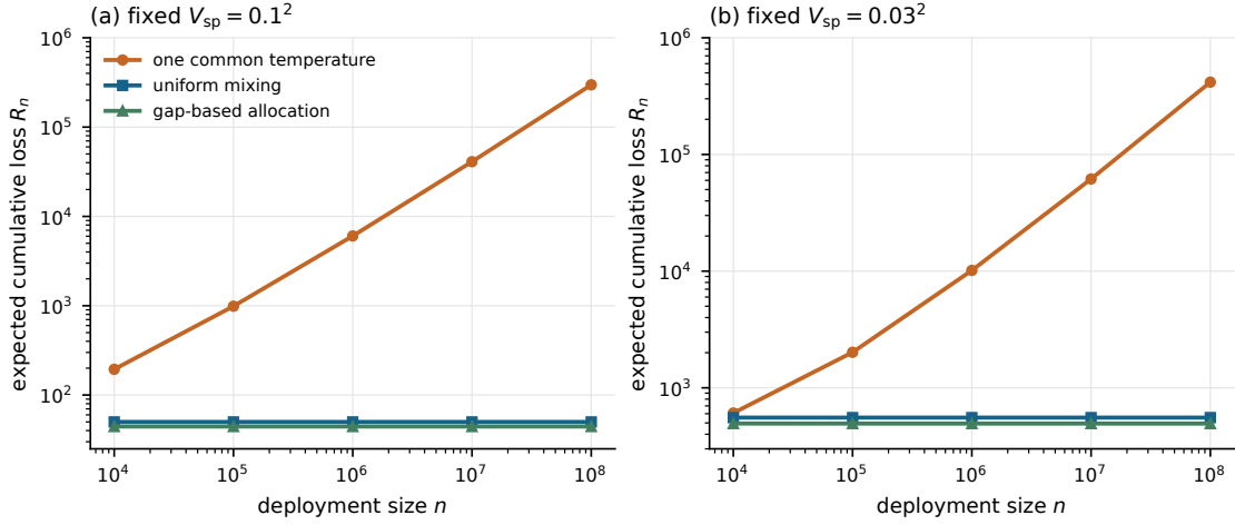
Figure 3: Exploration loss as deployment size increases, using the archived deterministic calculations with H \sim U(-1, 1) , g(h) = |h| , \sigma^2 = 1 , and fixed V_{sp} = \delta^2 . Curves share the same sparse-exploration criterion, not verified equal finite-sample MSE. Context-dependent temperature implements the gap-based probabilities and gives the same curve. The panels have different vertical ranges.
