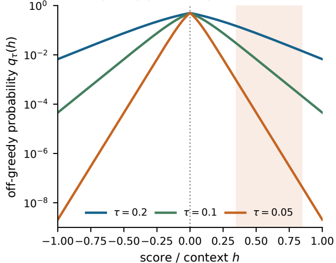
(b) off-greedy probability
