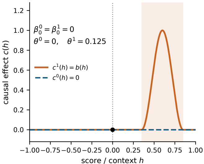
(a) same boundary, different population
