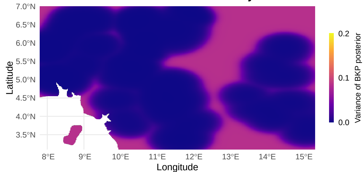
BKP – Prediction uncertainty
