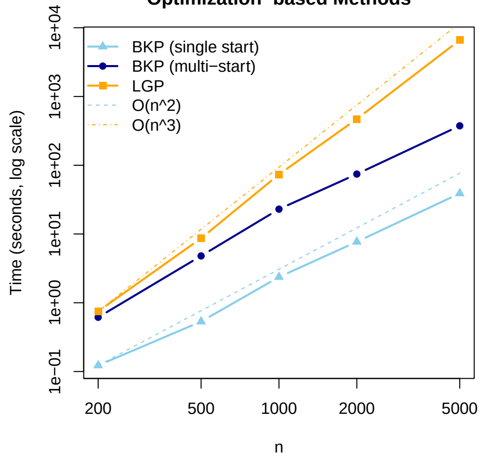
Optimization-based Methods
