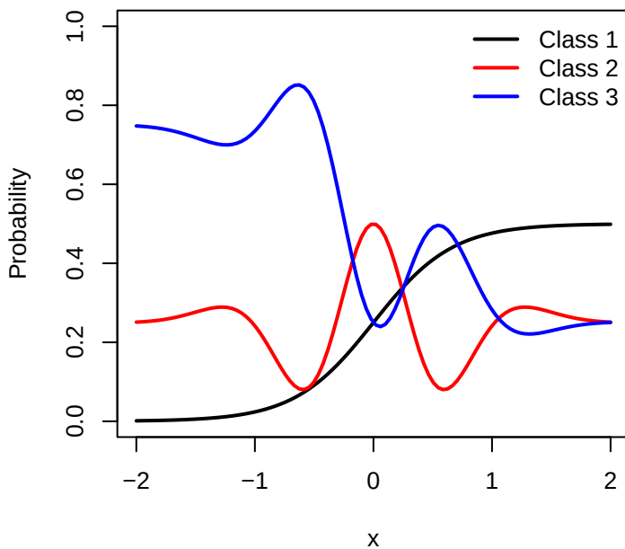
True Probability
