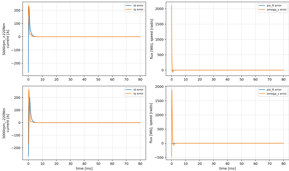
SLED 2023 Appendix A observer convergence
